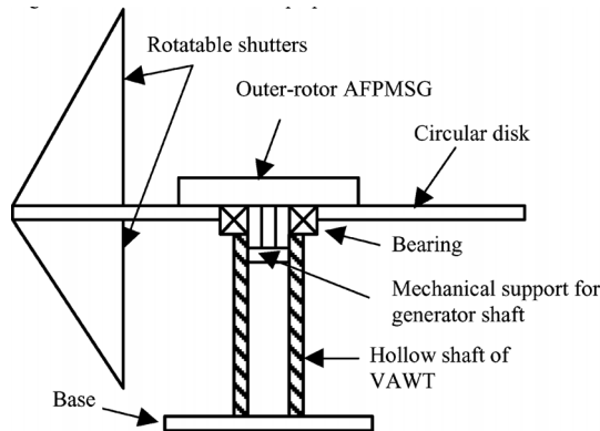
Fig. 18.11. Vertical-axis wind turbine (VAWT) using the proposed outer-rotor AFPMSG
