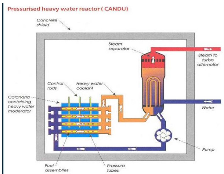
Figure 1.14 CANDU Reactor
