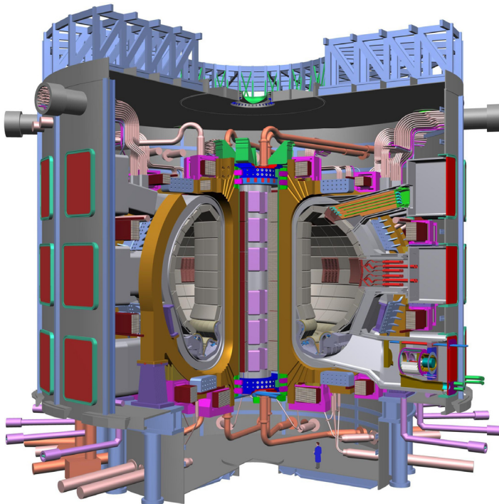
Figure 1.18 International Tokamak Experimental Reactor (ITER)
