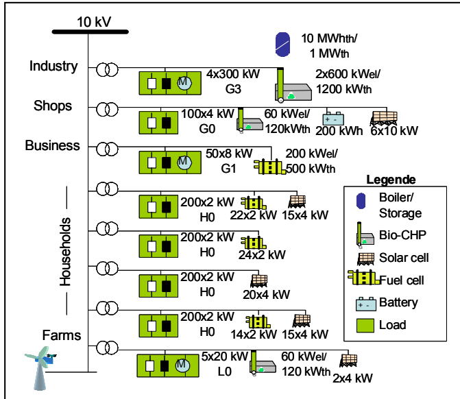
Fig. 8.12. Considered Distribution Network
