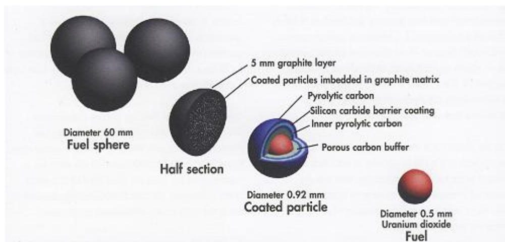
Figure 1.16 Fuel Element Design for PBMR
