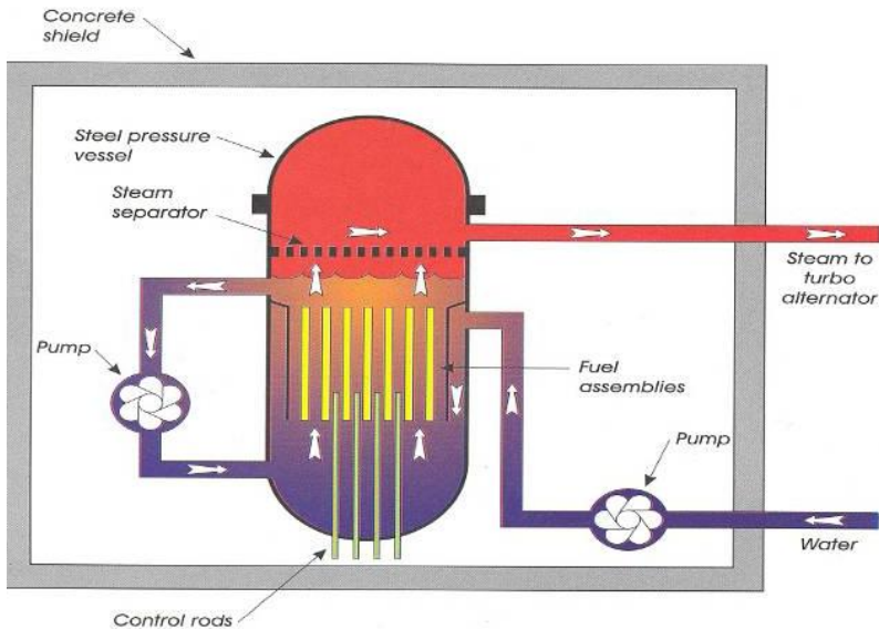
Figure 1.11 Boiling Water reactor (BWR)
