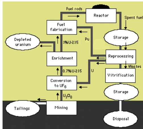
Figure 1.17 The Nuclear Fuel Cycle
