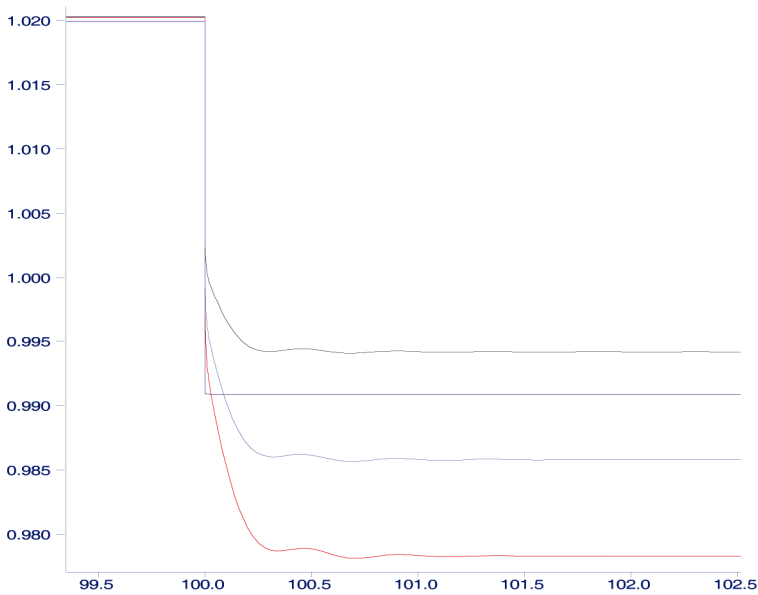
Fig. 8.8. Voltage Dip at Bus 2 with Induction Generator
