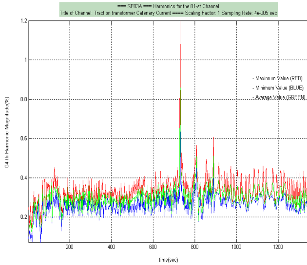
Fig. 18.4. Fourth harmonic
