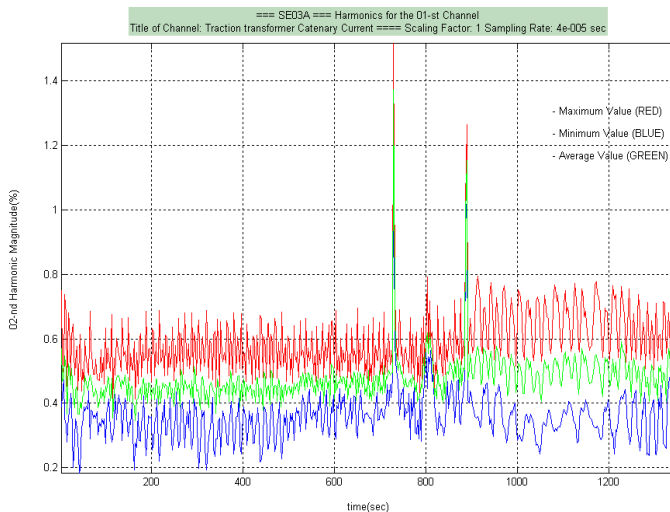
Fig. 18.2. Second harmonic
