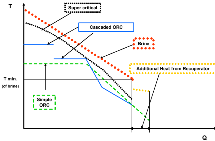
Fig. 5.7. Typical T/Q diagram
