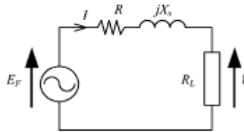
Fig. 18.19. Per-phase equivalent circuit of AFPMSG
