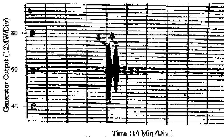
Figure 19.9(b). Real Power Oscillation
