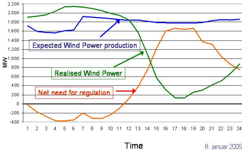
Fig. 8.19. Need for Regulation in Western Danish System during the Passing of a Wind Front
