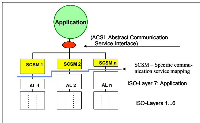
Fig. 8.14. Reference Model of IEC 61850
