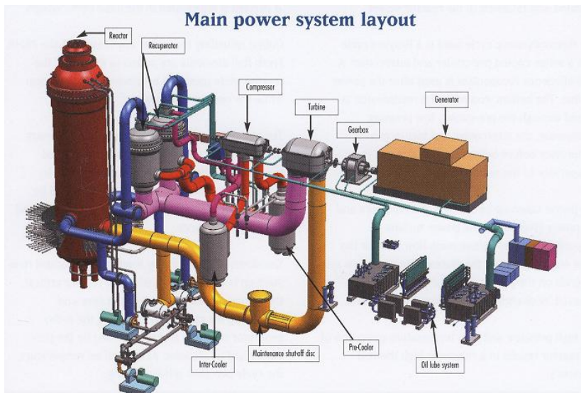
Figure 1.15 Pebble Bed Modular Reactor (PBMR)
