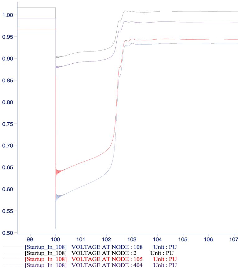
Fig. 8.9. Voltage Dip when an Induction Generator Starts Up
