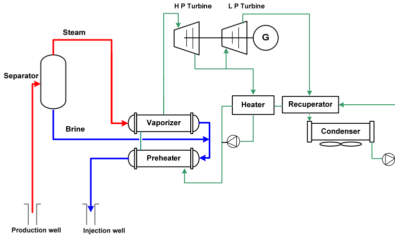
Fig. 5.10. Secondary organic loop cycle
