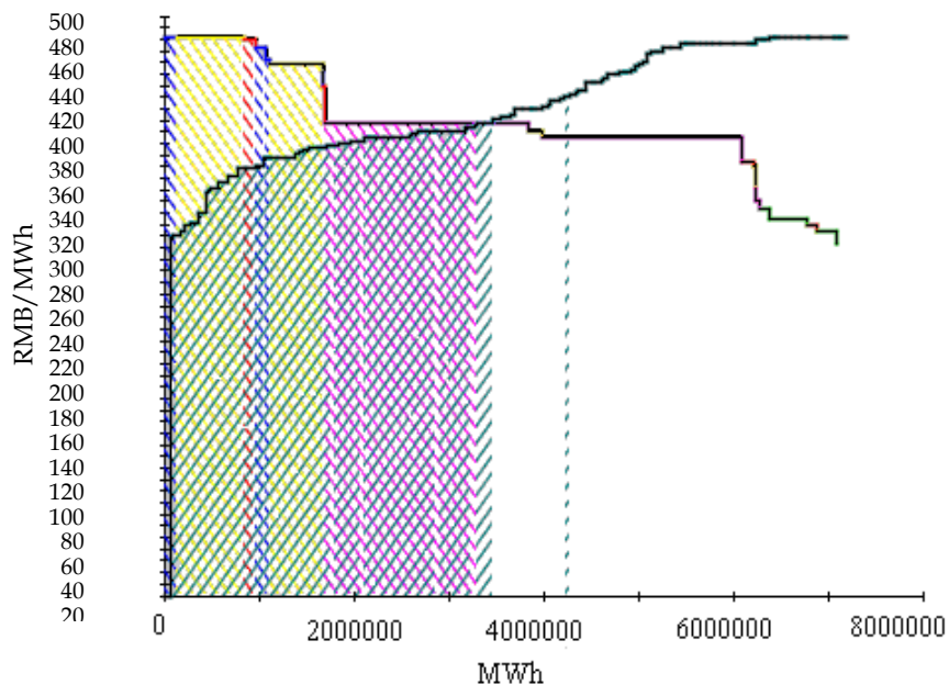
Figure 9.3 The merit curve of peak load time in June 2004
