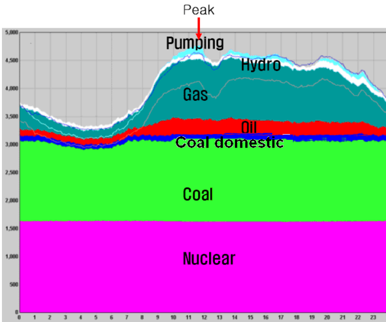
Figure 9.16 Hourly load curve for summer peak load on August 22, 2003.
