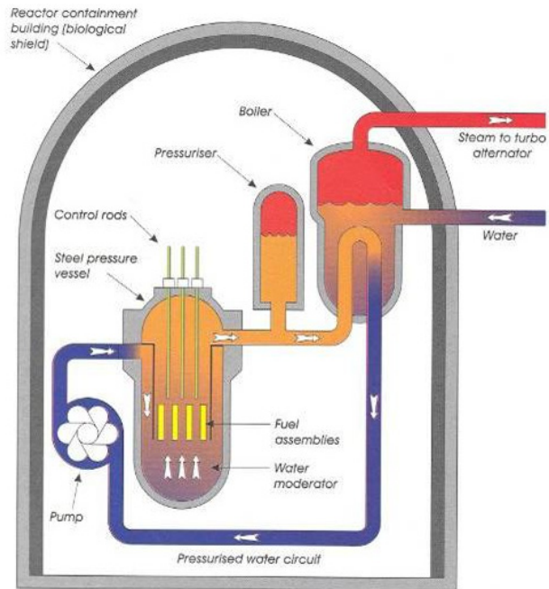
Figure 1.10 Pressurized Water Reactor (CPWR)
