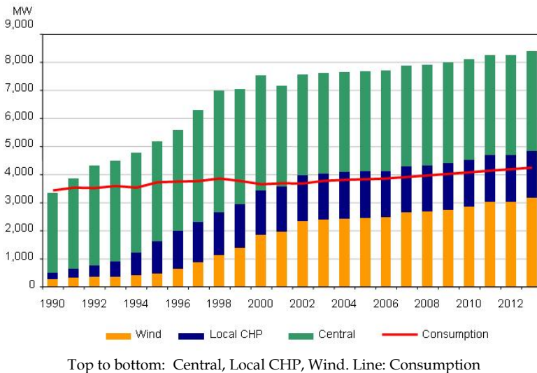
Fig. 8.18. Development of the Power Balance in Western Denmark
