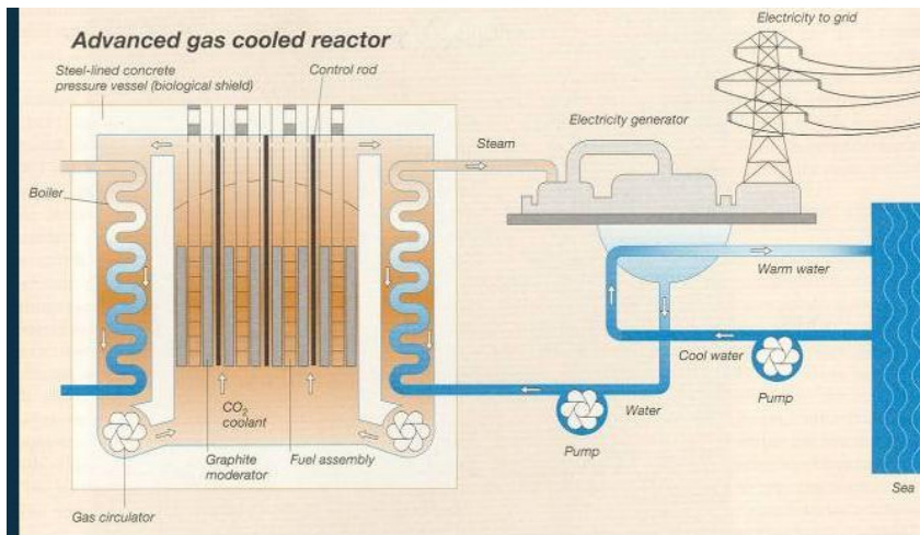
Figure 1.13 Advanced Gas Cooled Reactor (AGR)
