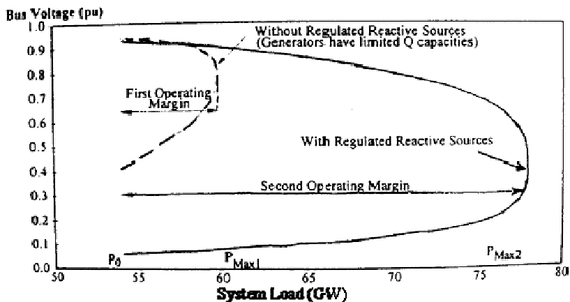
Figure 19.10. PV Curve of a Power System
