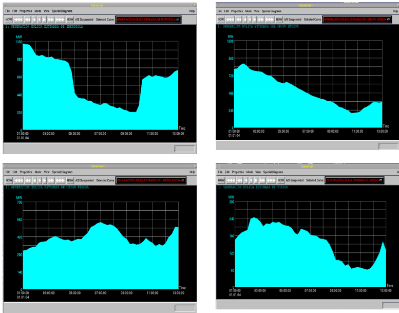
Figure 7.19. Wind Production in Four Different Distribution Areas
