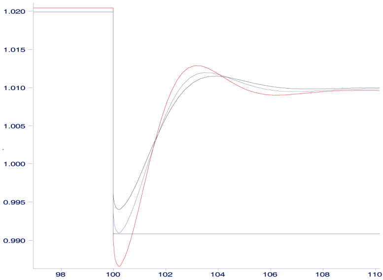
Fig. 8.7. Voltage Dip at Bus 2 with Synchronous Generator
