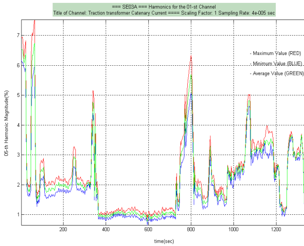
Fig. 18.5. Fifth harmonic
