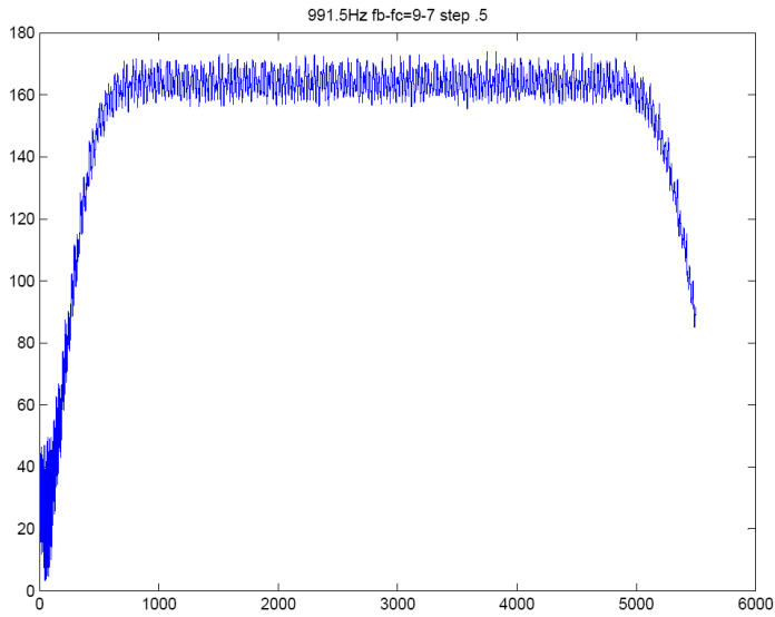
Fig. 18.7. Absolute coefficients plot generated by CWT (using Complex Morlet Wavelet, f_b=9 , f_c=7 ) for harmonic frequency at 991.5 Hz
