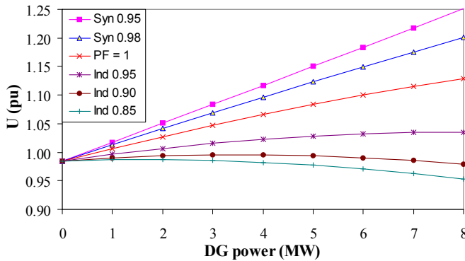
Fig. 8.4. Voltage at Node 406 with Different Power Factors
