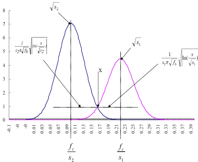
Fig. 18.6. Frequency plot of (14) for two CMWs at scales s_1 and s_2
