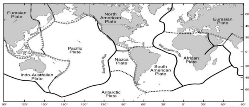
Fig. 5.2. Major Tectonic Plates of the World
