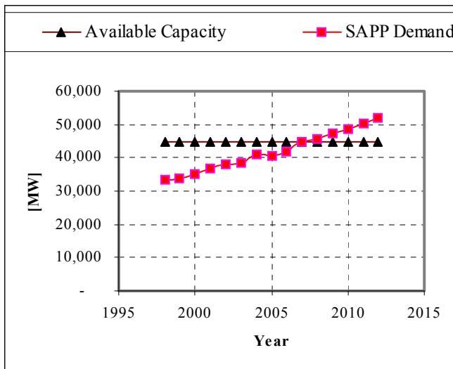
Fig. 10.5 Historic and forecast peak demand growth (1998 – 2012)
