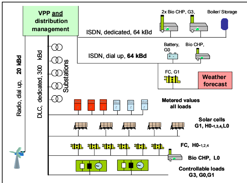
Fig. 8.15. Scheme of the Communication Network
