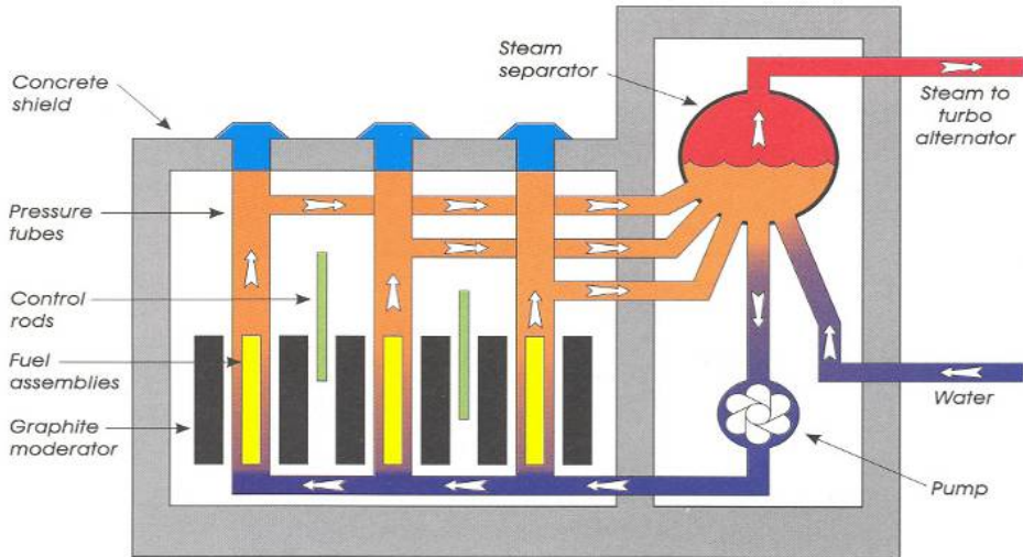
Figure 1.9 RBMK Reactors
