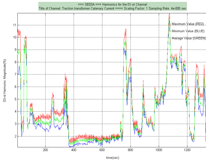
Fig. 18.3. Third harmonic
