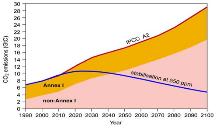
Figure 15.6. Depiction of CO 2 emission reductions required to stabilize at 550ppm
