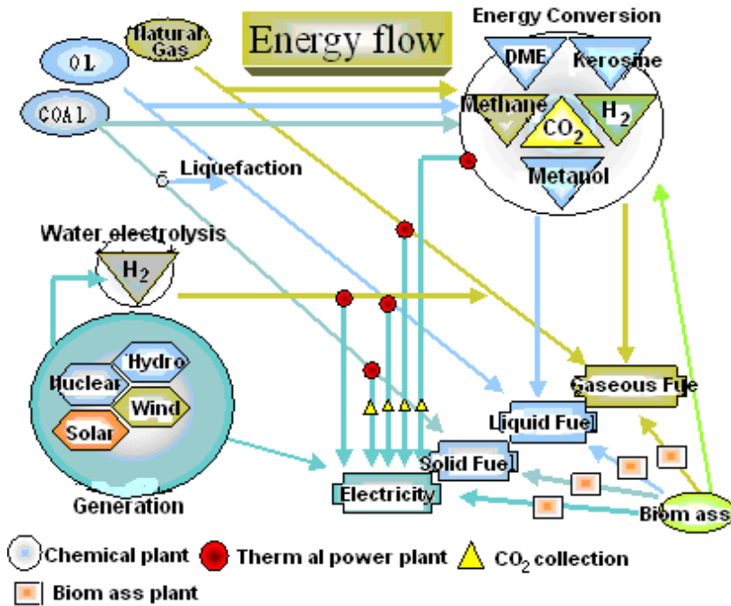
Fig. 11.4 Configuration of the energy system of each node of the model
