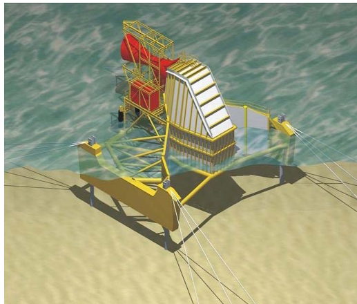
Fig. 4.6. Energetech WEC device.
