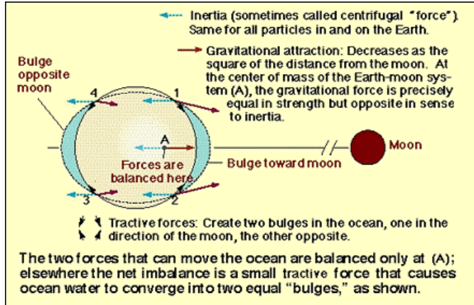
Fig. 4.3. Tide-generating forces based on earth-moon interactions.
