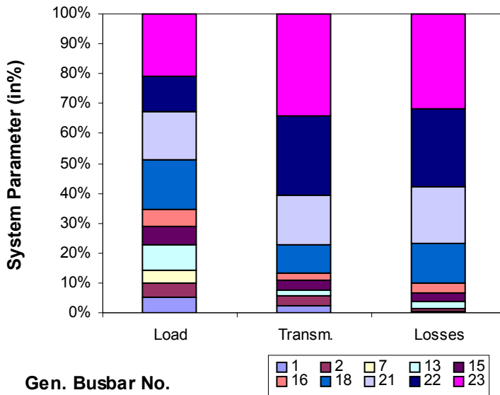
Fig. 6.3. Relative contributions of each generating unit output to system load, transmission use and losses (Case 3)
