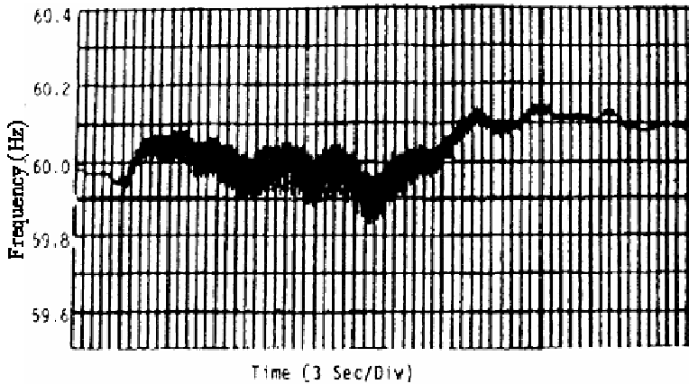
Figure 19.9(a). System Frequency Oscillation
