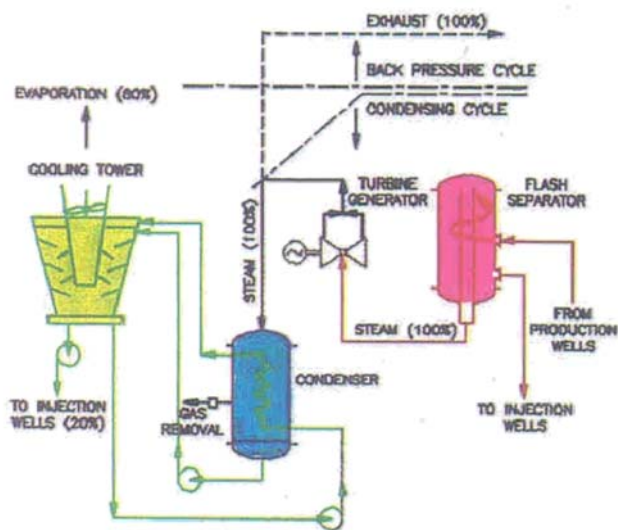
Fig. 5.6. Conventional geothermal power plant - Backpressure or condensing
