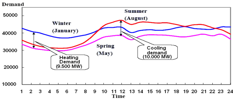
Figure 9.15 Seasonal load-demand pattern
